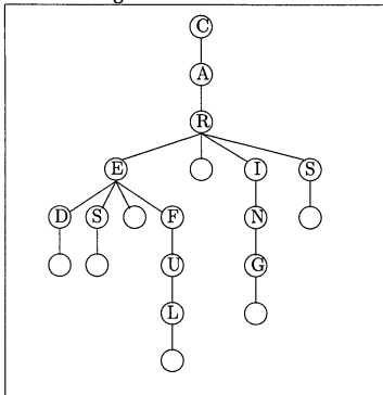
Figure 2: Trie structure
