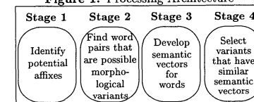
Figure 1: Processing Architecture
